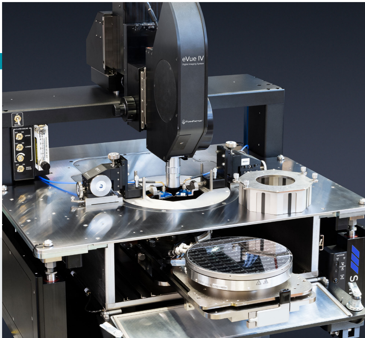
Summit 11000
